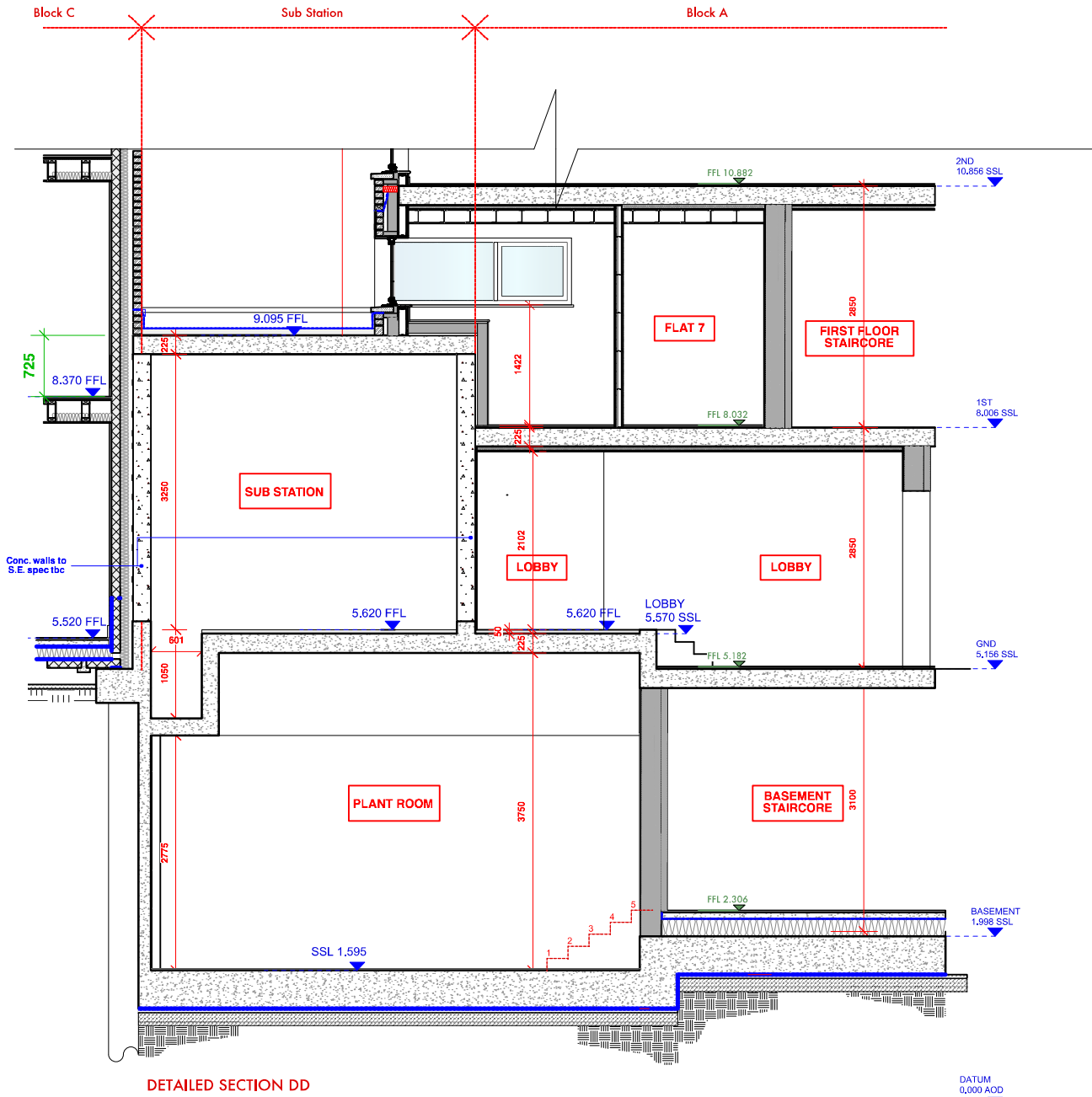
DETAILED SECTION DD SCALE 1:50 @ A3
