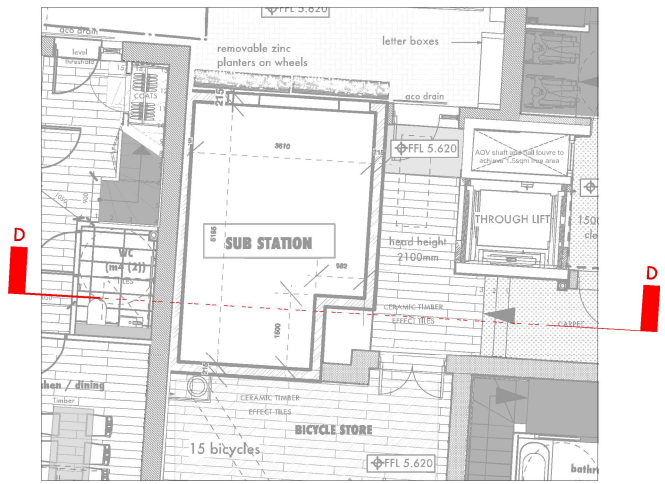
PARTIAL FLOOR PLAN BLOCK A 1:100 @ A3
